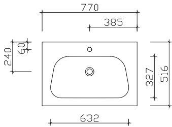
Breite 770 mm BME001M77001
